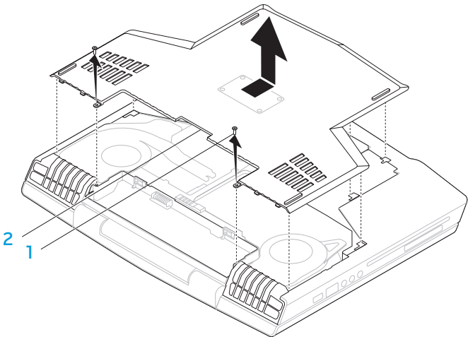
2 compartment door
